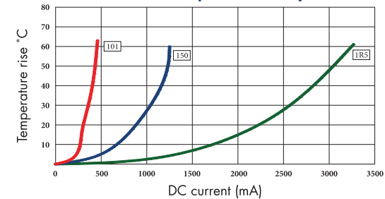
OWIRH3D16A Temperature rise by current
