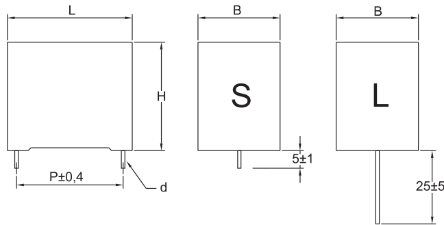
2 terminals execution
