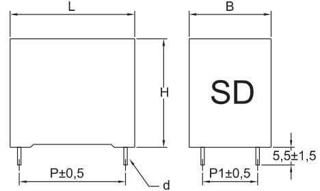
4 terminals execution
