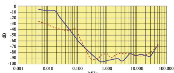
FL 155.250.00 250 A
