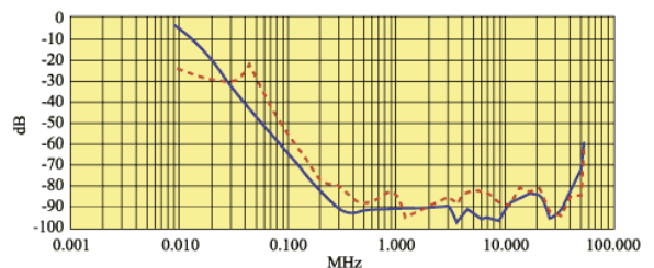
FL 155.50.00 50 A
